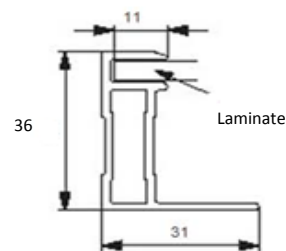
Solaire Direct frame Profile
